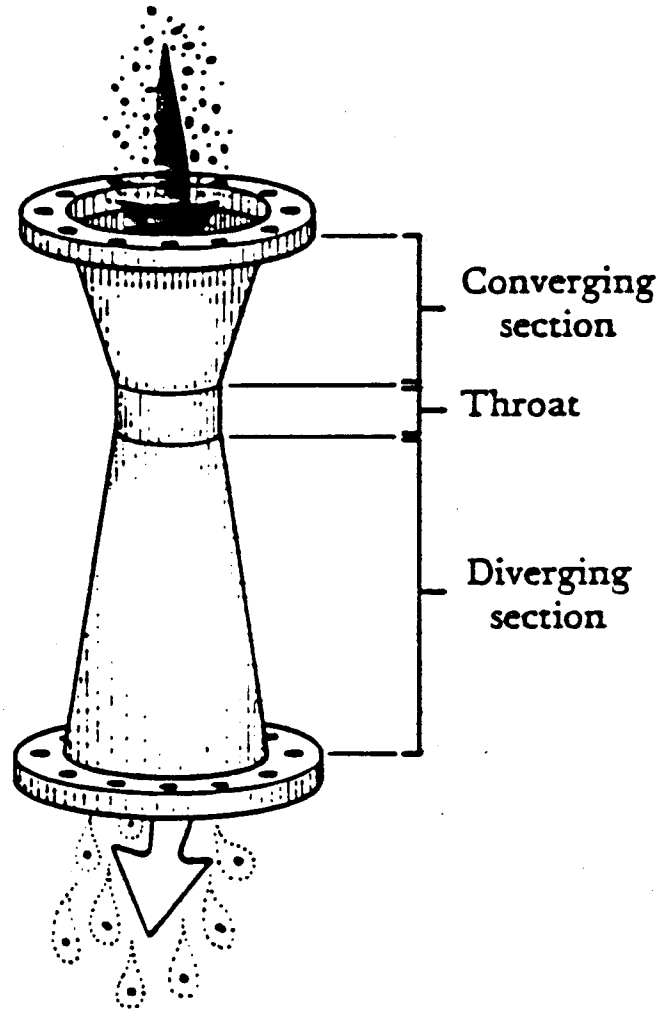
Figure 3-2. Spray venturi with circular throat. 6
