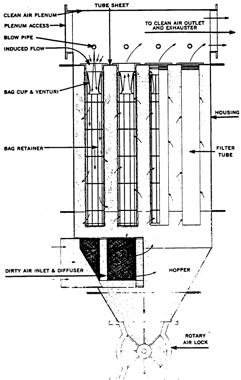
Figure 3-6. Pulse jet baghouse. 12
