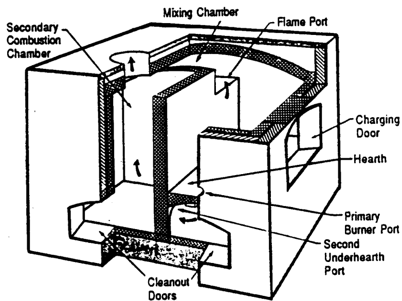
Figure 2-4. Retort multiple-chamber incinerator for pathological wastes.
