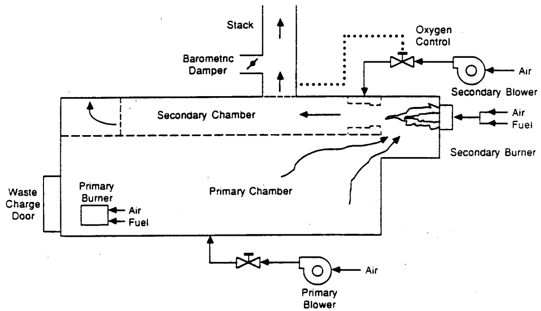
Figure 2-6. Schematic of a single batch controlled-air incinerator. 17
