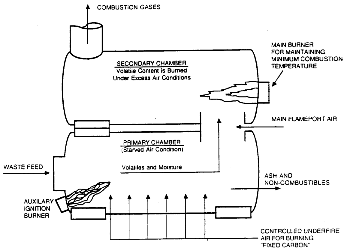
Figure 2-5. Schematic of a controlled-air incinerator. 16
