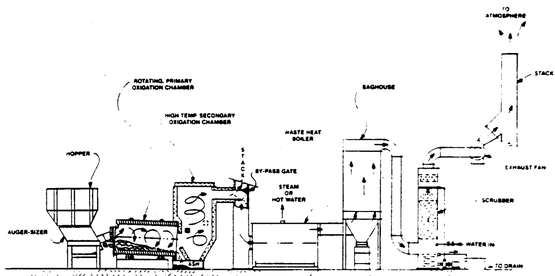
Figure 2-10. Rotary kiln with auger feed. 22
