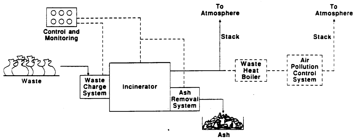
Figure 2-1. Major components of an incineration system.
